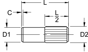
Half-Length Offset Straight Knurl Series KP120
