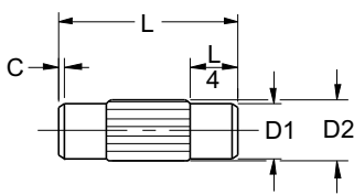
Half-Length Centered Straight Knurl Series KP110
