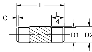
Half-Length Centered Helical Knurl Series KP210
