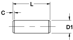
Straight Pin Series DP100
