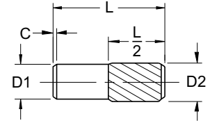
Half-Length Offset Helical Knurl Series KP220
